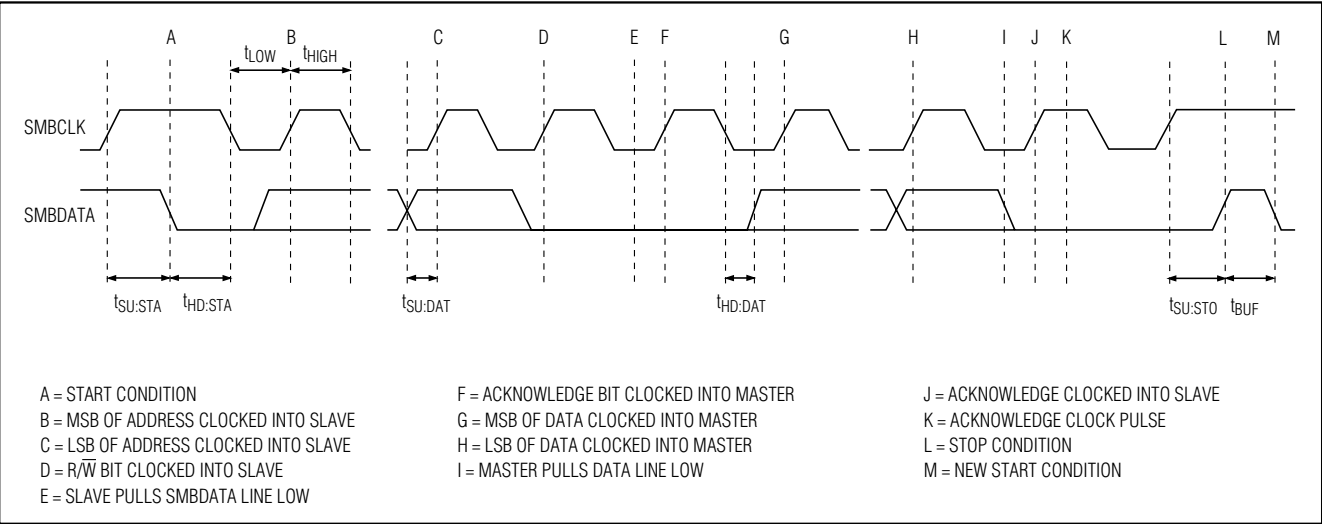
Figure 4. I²C/SMBus Read Timing Diagram
