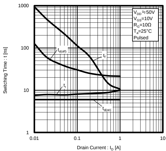
Fig.11 Switching Characteristics
