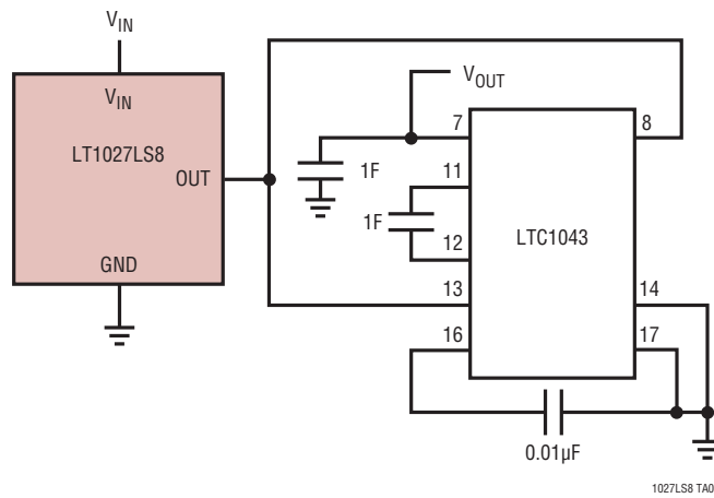
10V Reference
