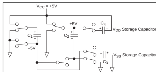
Figure 3. Charge Pump Phase 1 for \pm 5V .
