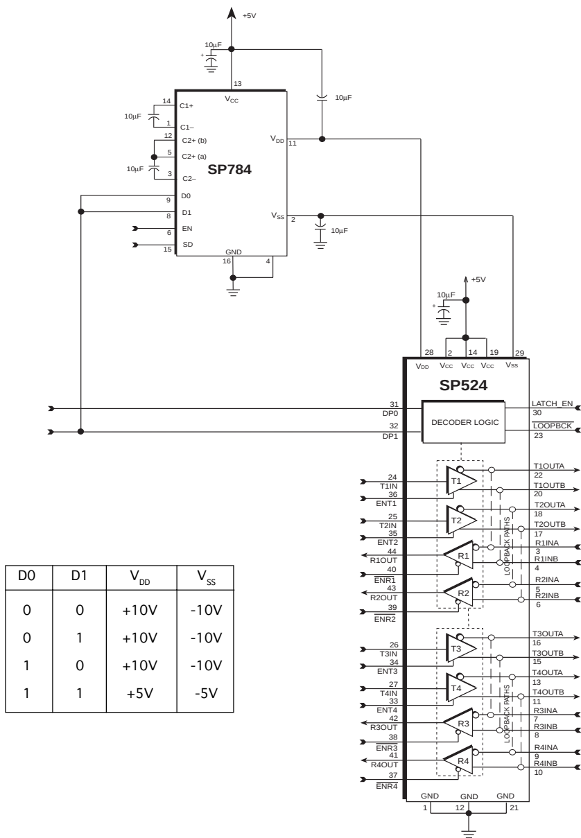
Figure 8. SP784 Application w/ SP524 Multi-Protocol Transceiver IC.
