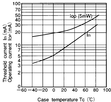
Fig.2 Temperature dependence of I_{th} and lop
