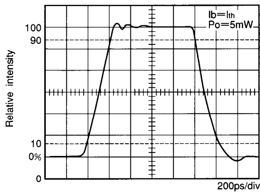
Fig.8 Pulse response characteristics
