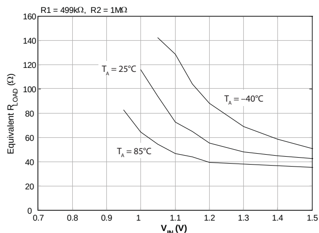
Startup Min. Load Resistance vs. V_{IN} ( V_{OUT} = 1.8V )
