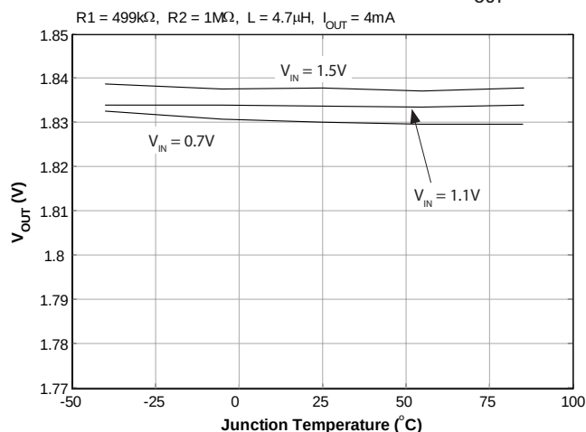
Temperature Reg. — PSAVE Mode ( V_{OUT} = 1.8V )
