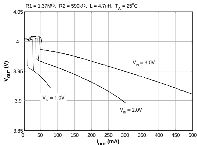
Load Regulation vs. ( V_{OUT} = 4.0V )
