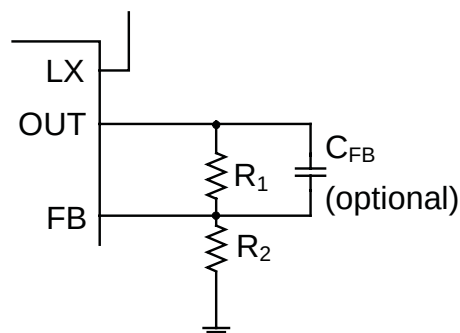
Figure 1 — Output Voltage Feedback Circuit
