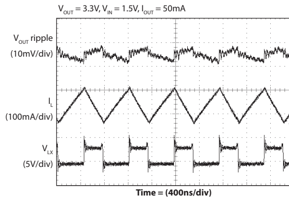
PWM Operation
