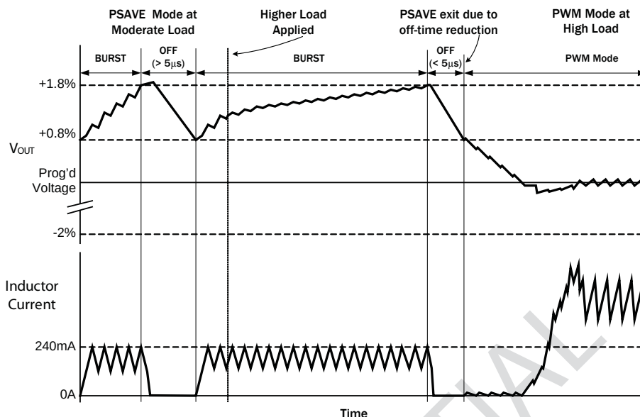
Figure 3 — PSAVE Operation With Exit to PWM Due To Off-time < 5μs
