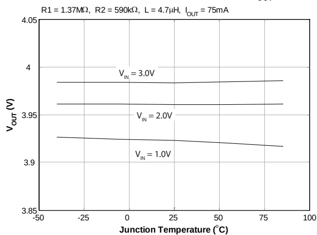
Temperature Reg. — PWM Mode ( V_{OUT} = 4.0V )
