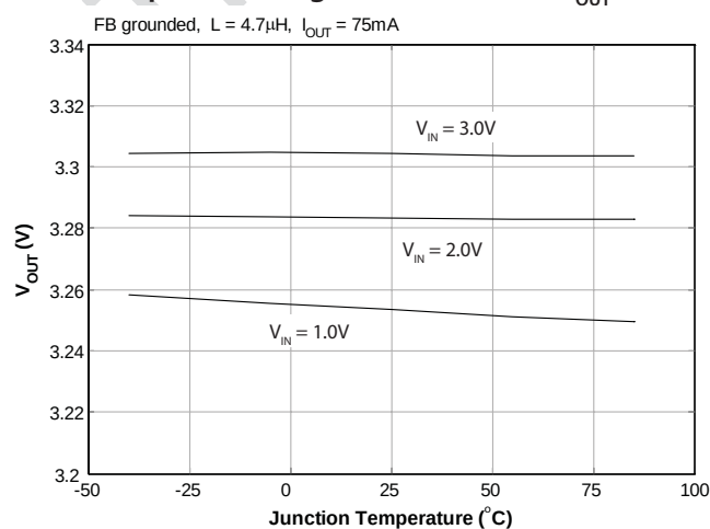
Temperature Reg. — PWM Mode ( V_{OUT} = 3.3V )
