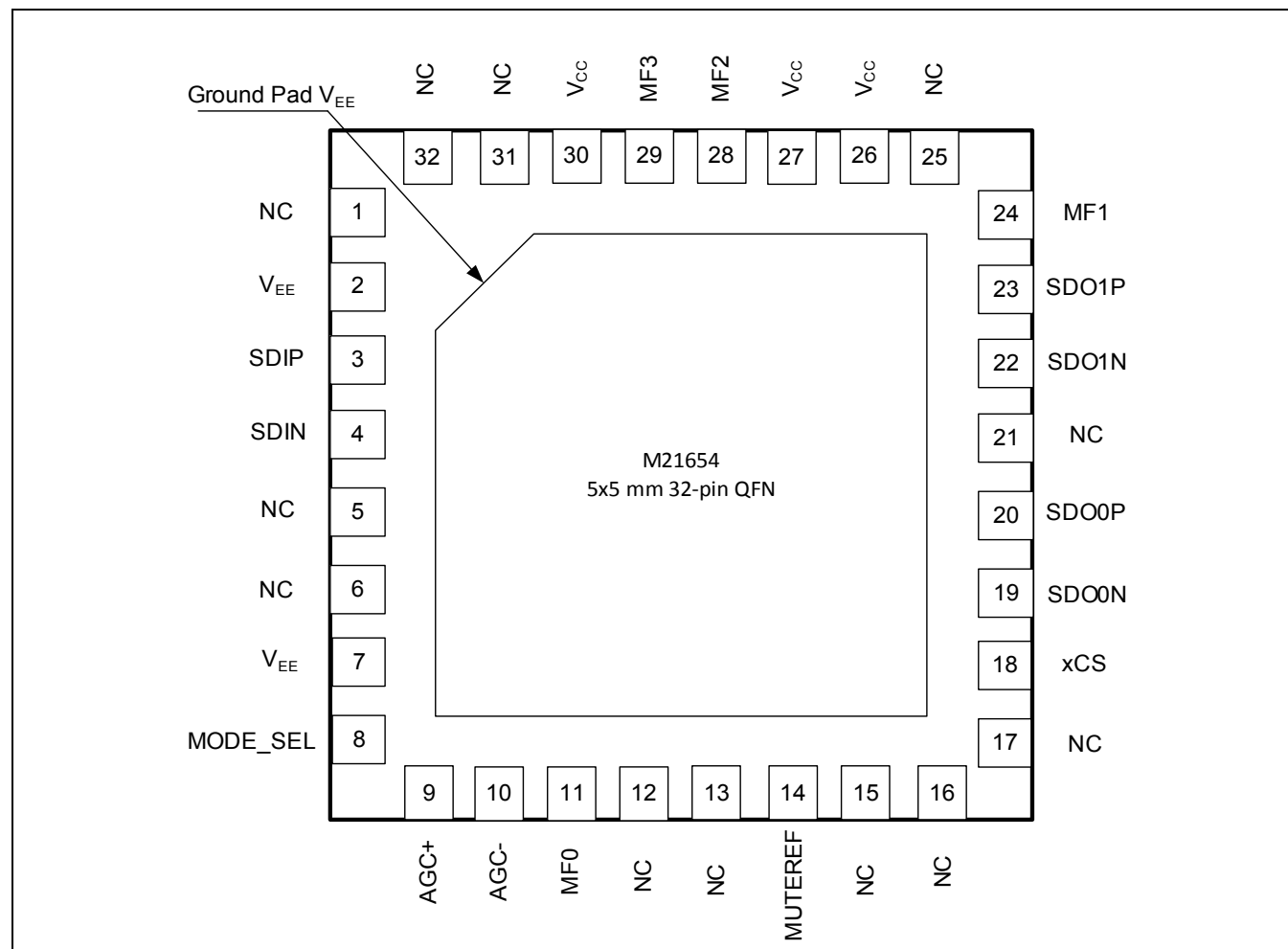
Figure 3-3. M21654 Pinout Diagram (Bottom View of the Package)
