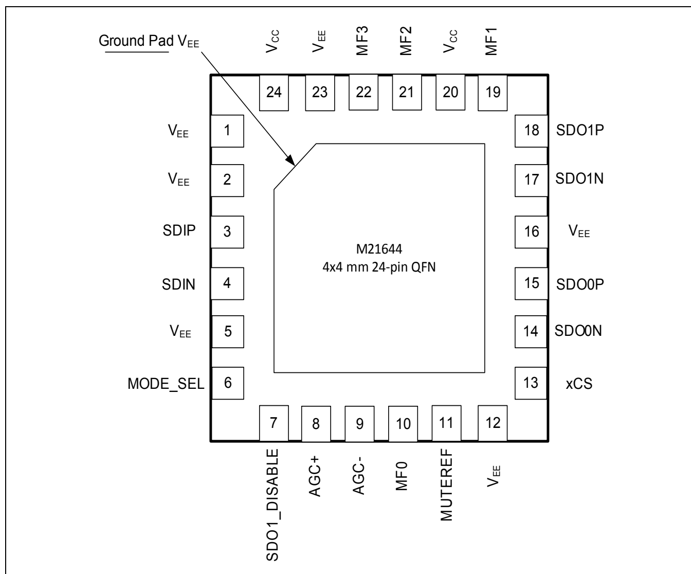
Figure 3-1. M21644 Pinout Diagram (Bottom View of the Package)
