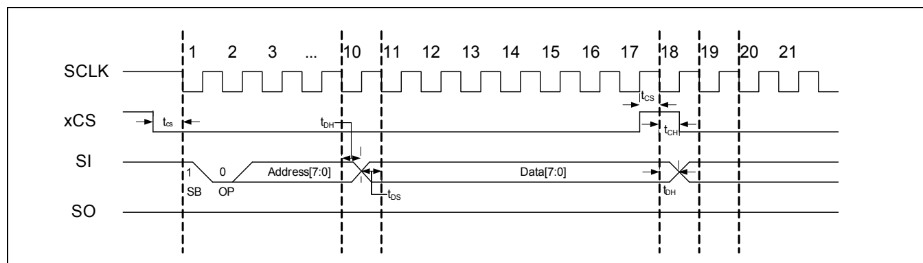
Figure 4-4. 4-wire Random WRITE Timing Diagram
