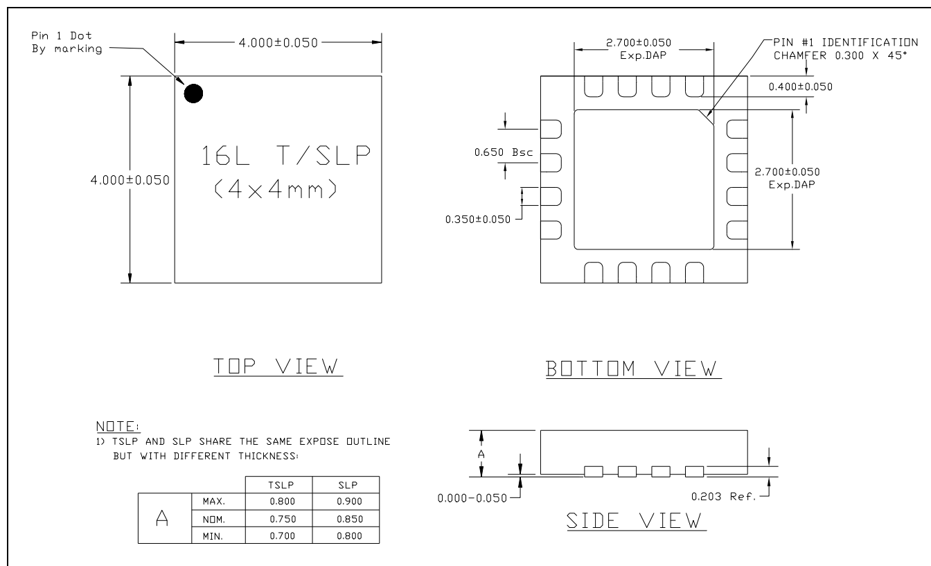
Figure 3-6. M21664 Packaging Drawing
