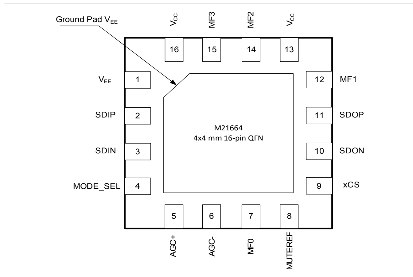
Figure 3-5. M21664 Pinout Diagram (Bottom View of the Package)
