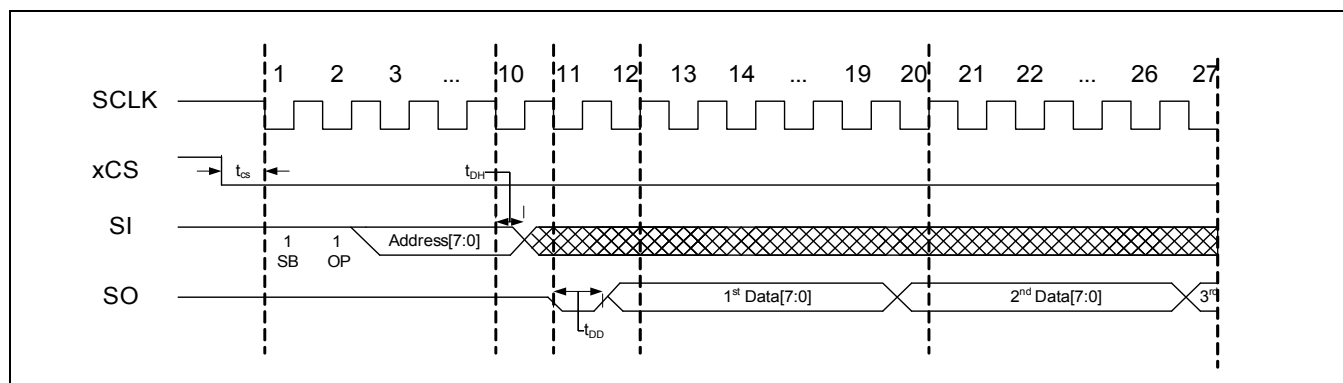
Figure 4-7. 4-wire Sequential READ Timing Diagram
