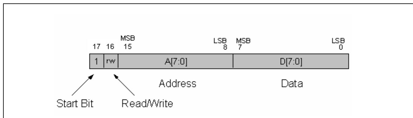
Figure 4-3. 4-wire Serial Digital Interface
