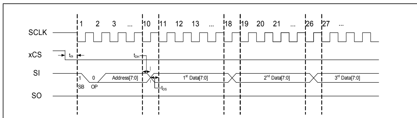
Figure 4-5. 4-wire Sequential WRITE Timing Diagram
