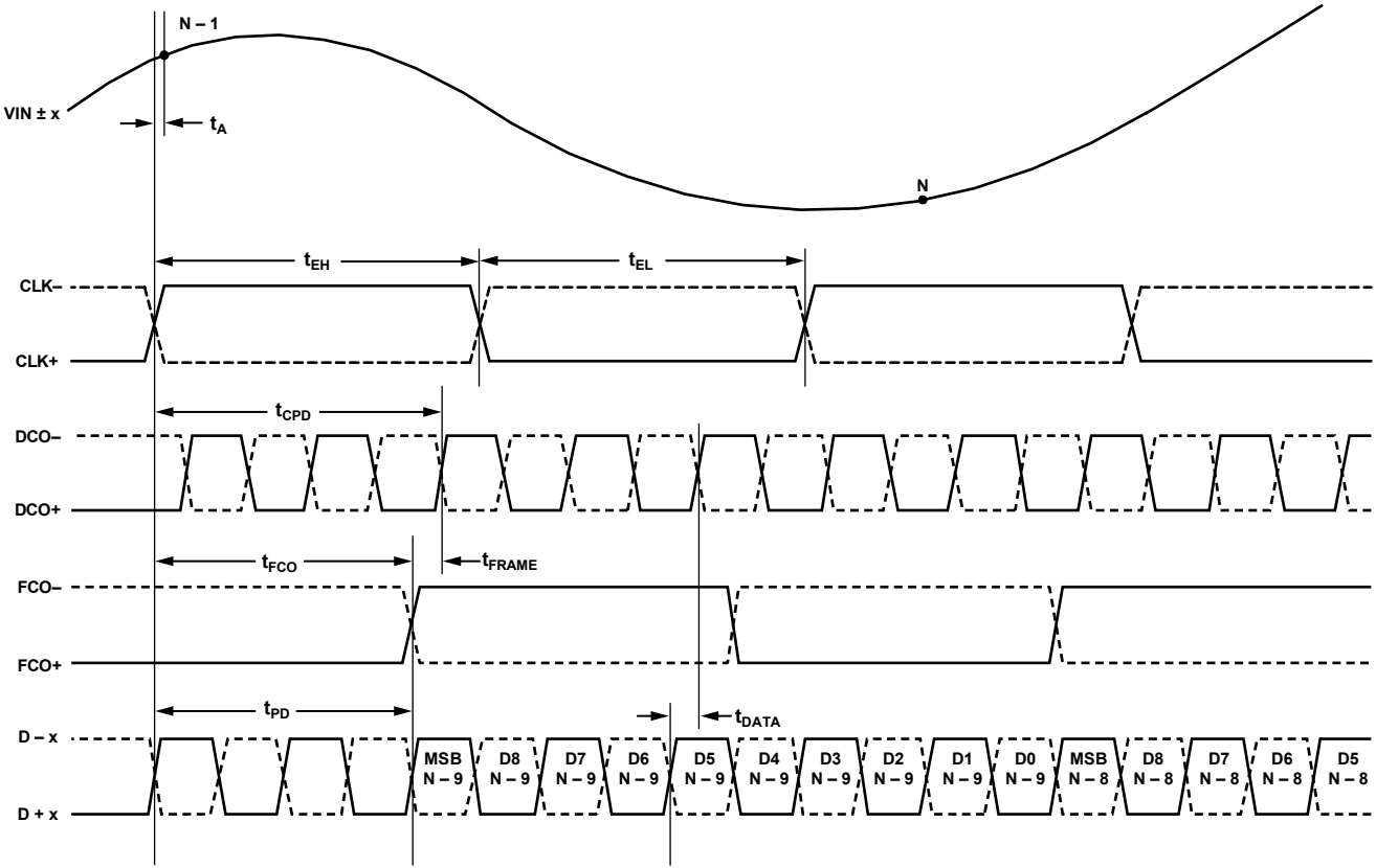
Figure 2. 10-Bit Data Serial Stream (Default), MSB First
