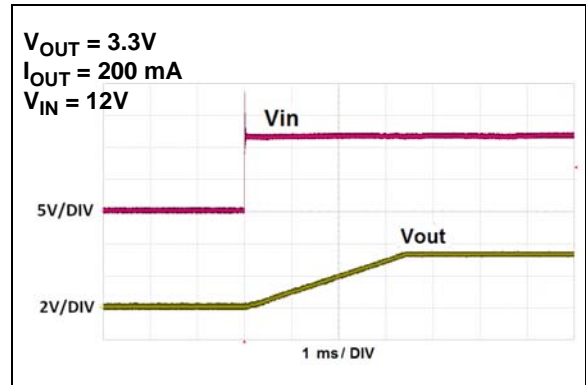
FIGURE 2-29: Startup From V_{IN} .
