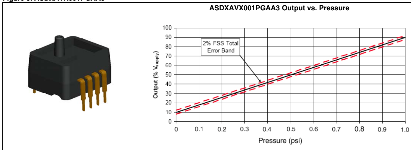
Figure 3. ASDXAVX001PGAA3
