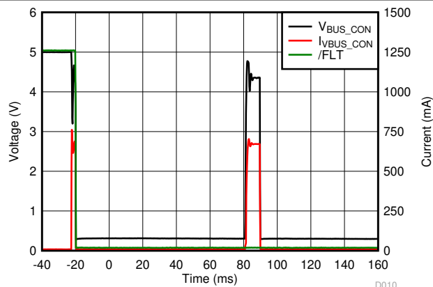
图 6-8. Overcurrent t_{\text{BLANK\_RETRY}} Response Waveform
