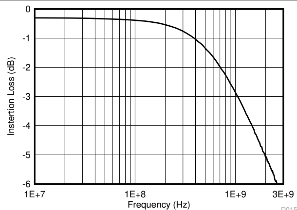
图 6-17. Data Switch Differential Bandwidth
