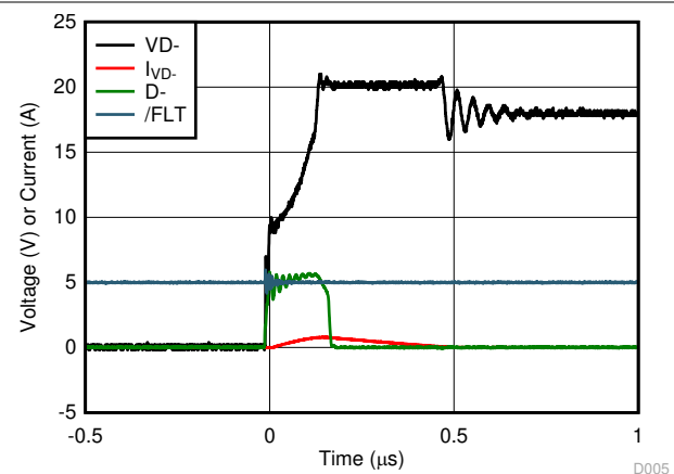
图 6-12. Data Switch Short-to-18 V Response Waveform
