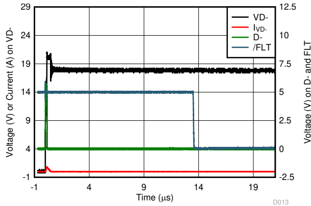
图 6-13. Data Switch Short-to-18 V Response Waveform (Long)
