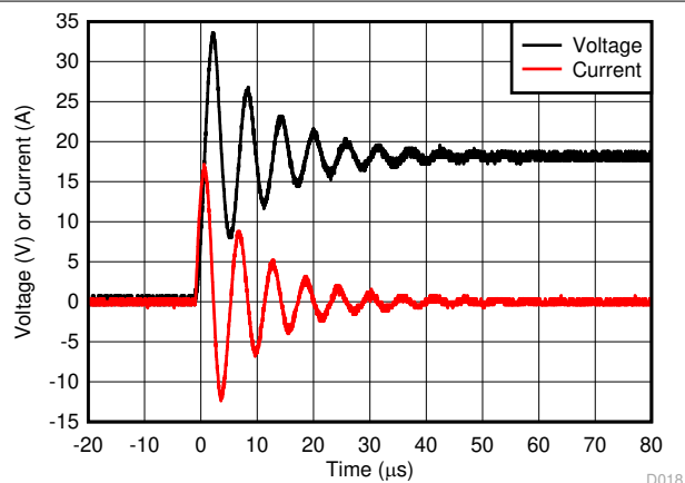
图 9-6. TPD3S716-Q1 and 100-V, 1-μF X7R Shorted to 18 V (Powered Off)
