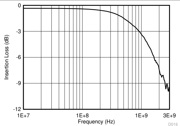
图 6-18. Data Switch Single-Ended Bandwidth
