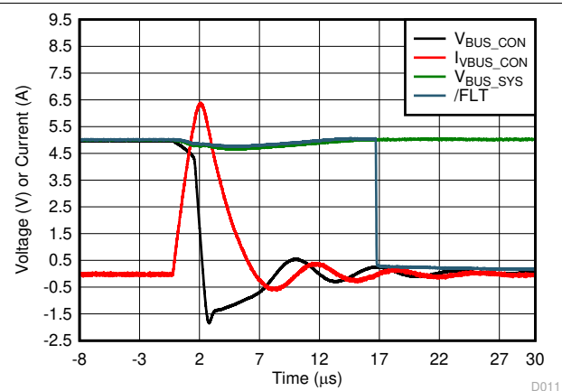
图 6-9. V_{\text{BUS}} Short-to-Ground Response Waveform
