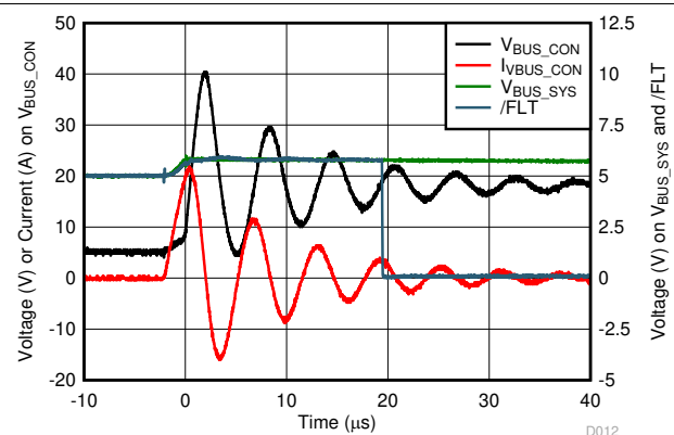
图 6-10. V_{\text{BUS}} Short-to-18 V Response Waveform
