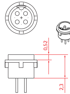
[10] STYLE 10
