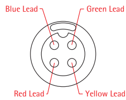
[ 4 ] 4 TERMINALS
