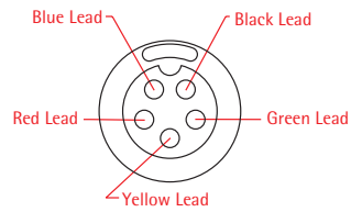
[ 5 ] 5 TERMINALS
