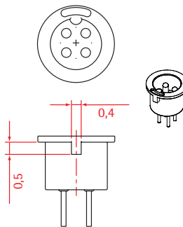
[05] STYLE 05
