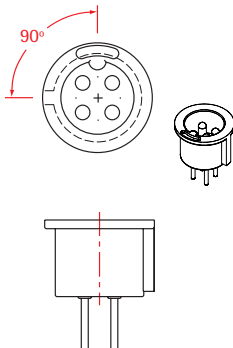
[08] STYLE 08
