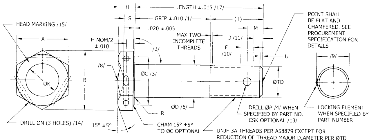
FIGURE 1 - BOLT CONFIGURATION
