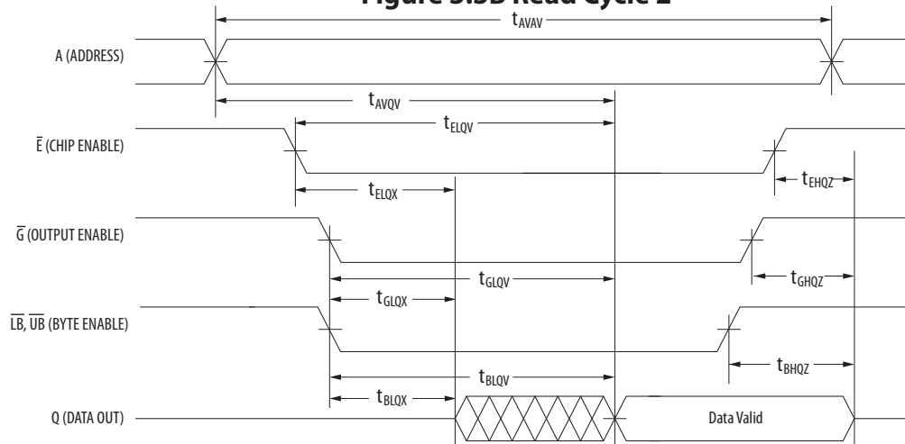
Figure 3.3B Read Cycle 2
