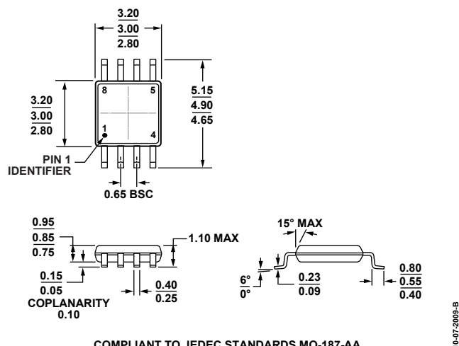
Figure 42. 8-Lead Mini Small Outline Package [MSOP] (RM-8)
