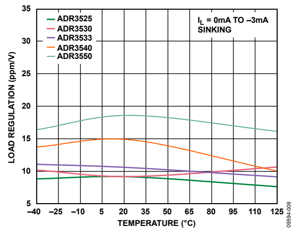
Figure 8. Load Regulation vs. Temperature (Sinking)
