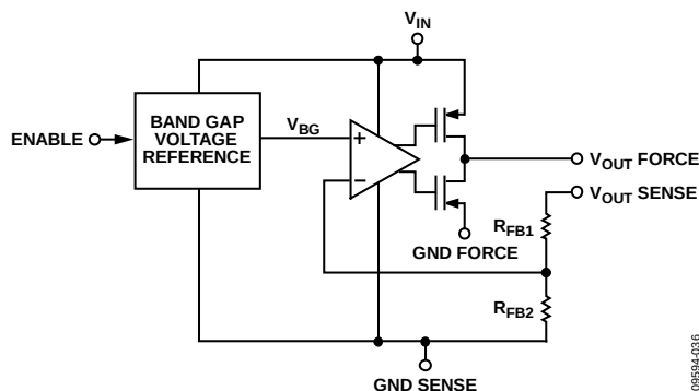
Figure 36. Block Diagram
