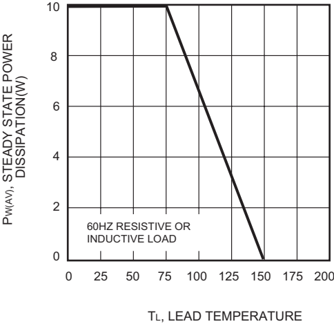
FIG.4 - STEADY STATE POWER DERATING CURVE
