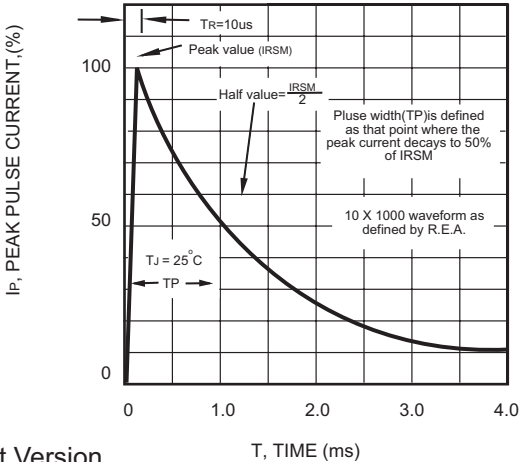
FIG.5 - PULSE WAVEFORM
