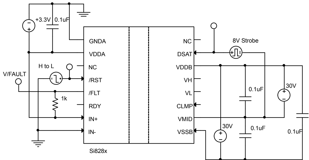
Figure 4.2. Si828x RST FLT CLEAR Test Circuit
