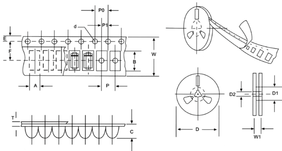
FIG:CONFIGURATION OF AXIAL TAPING
