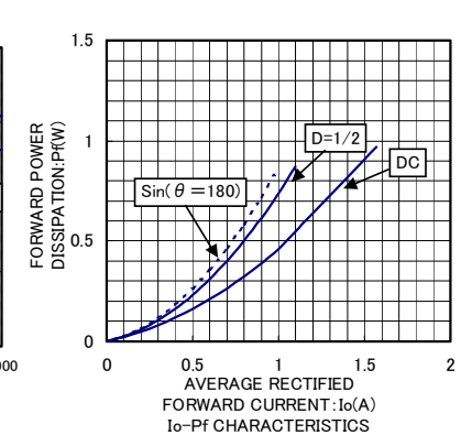
Io-Pf CHARACTERISTICS
