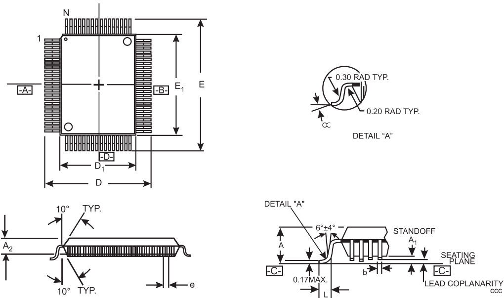
PQFP Package
