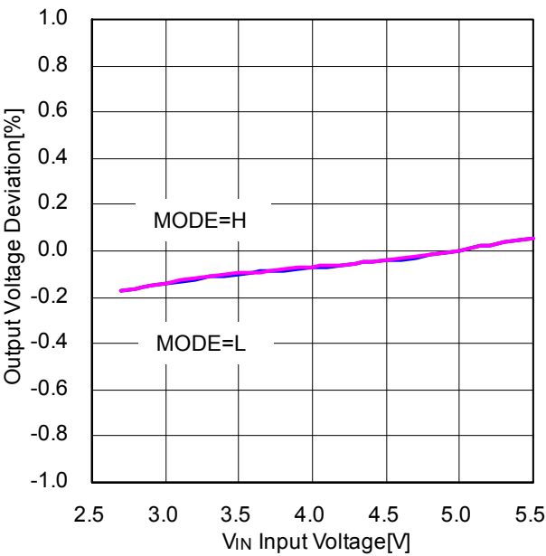
Figure 36. Line Regulation (VOUT=1.2V, L=1.5μH, FREQ=H, IOUT=2A)
