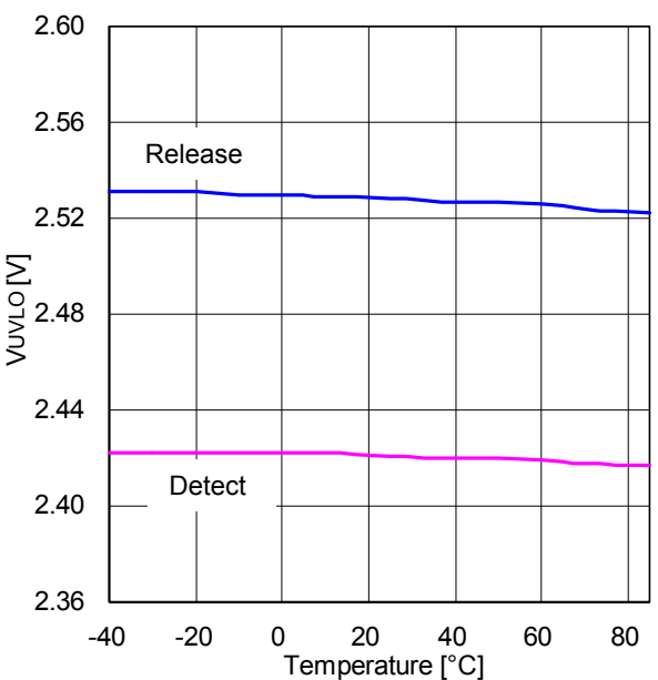
Figure 11. UVLO Threshold vs Temperature
