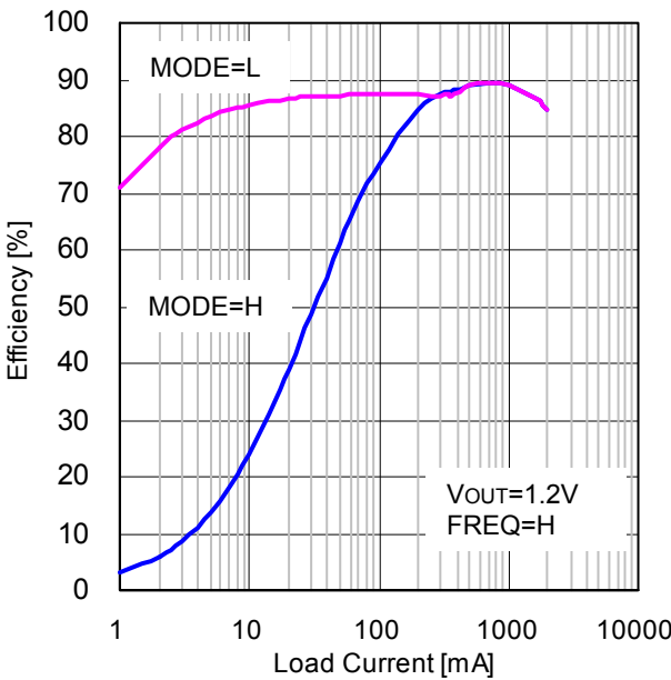
Figure 7. Efficiency vs Load Current (VIN=5V, VOUT=1.2V, L=1.5uH, FREQ=H)
