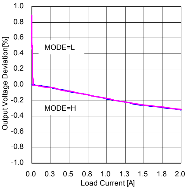
Figure 37. Load Regulation (VIN=5V, VOUT=1.2V, L=1.5μH, FREQ=H)
