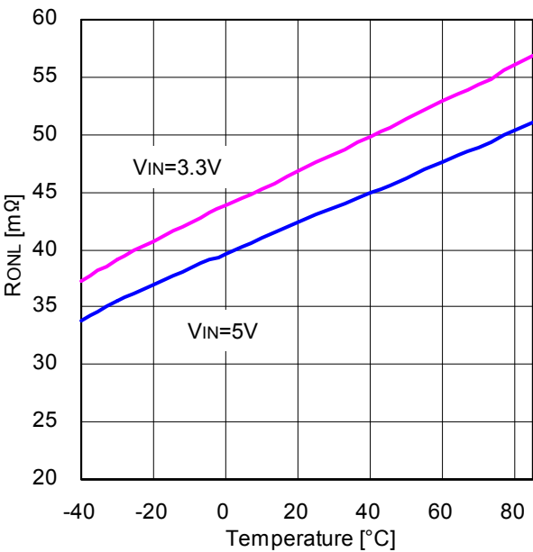
Figure 19. Low Side ON-Resistance vs Temperature
