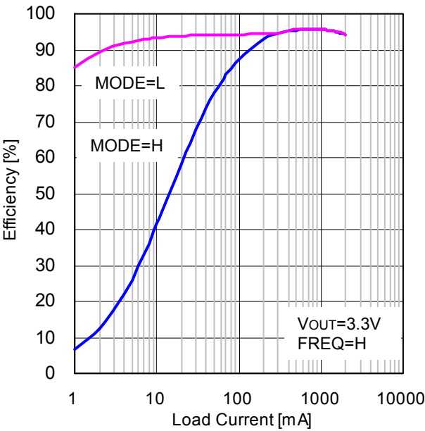
Figure 9. Efficiency vs Load Current (VIN=5V, VOUT=3.3V, L=1.5μH, FREQ=H)
