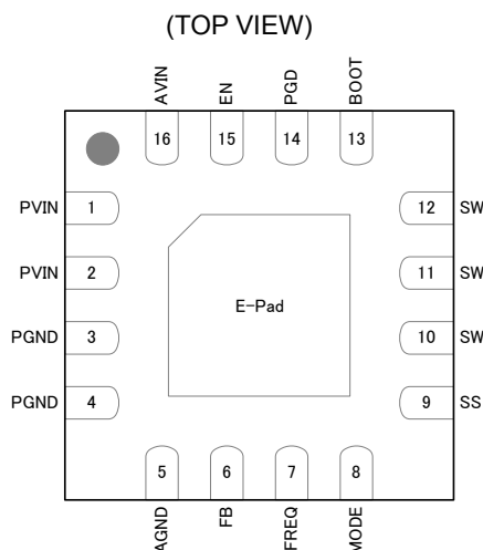
Figure 2. Pin Assignment
