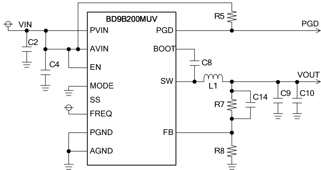
Figure 48. Application Circuit
