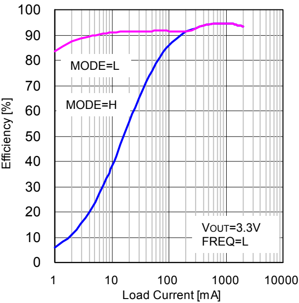
Figure 8. Efficiency vs Load Current (VIN=5V, VOUT=3.3V, L=1.0μH, FREQ=L)
