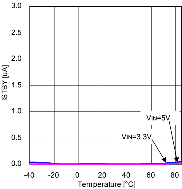
Figure 5. Stand-by Supply Current vs Temperature
