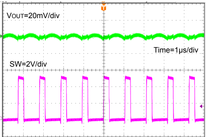
Figure 35. Switching Waveform (VIN=5V, VOUT=1.2V, FREQ=H, IOUT=2A)
