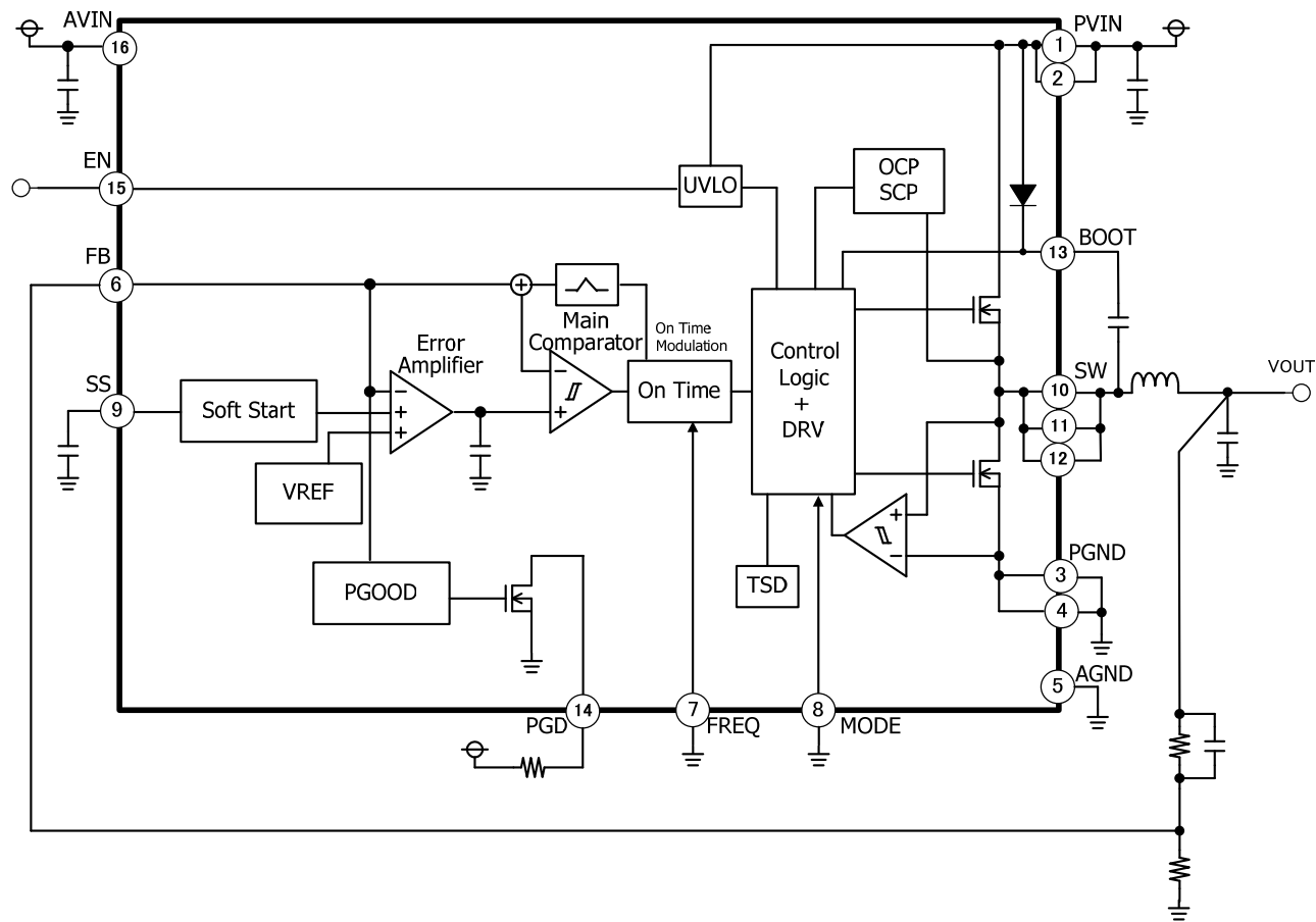
Figure 3. Block Diagram
