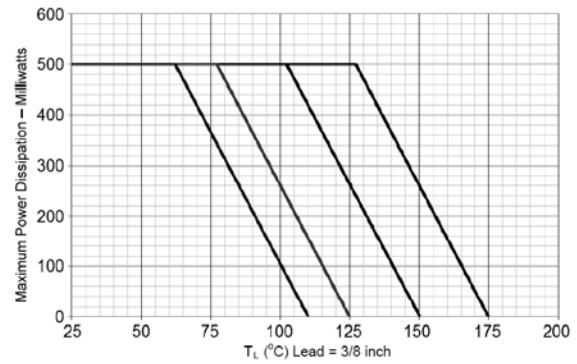
FIGURE 2 - (1N6321 – 1N6355) T_L Temperature-Power Derating Curve R_{\theta JA} 3/8 inch = 95.5 °C/W (dc operation)
