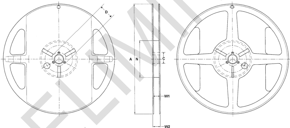
Figure 6 - Reel drawing
