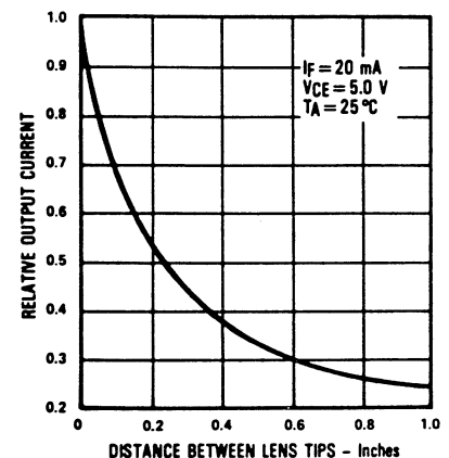
Coupling Characteristics of OP265W and OP505W
