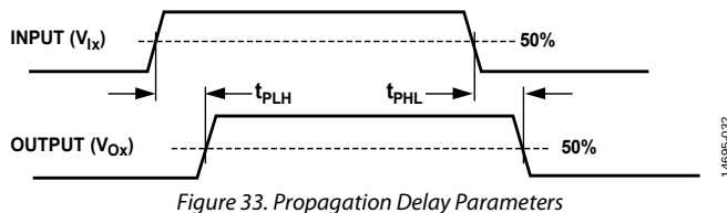
Figure 33. Propagation Delay Parameters
