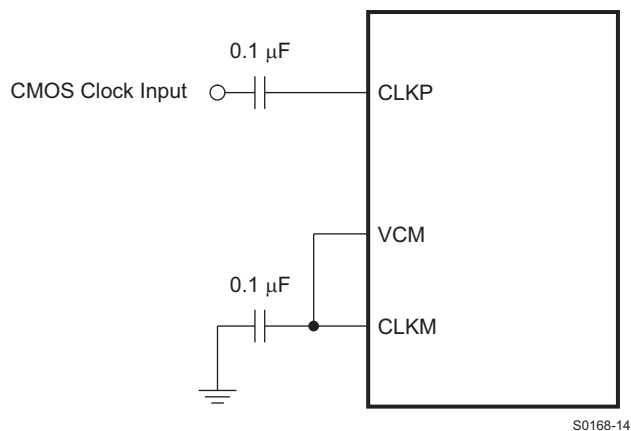
Figure 59. Single-Ended Clock Driving Circuit
