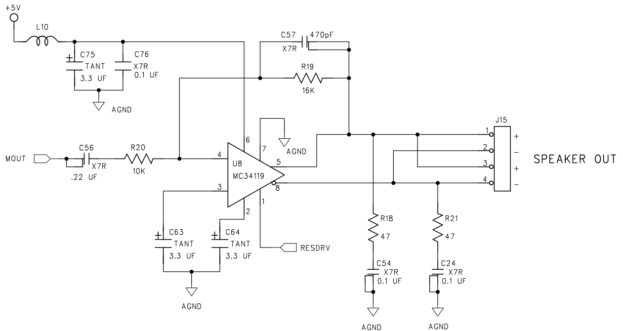
Figure 2. Microphone In
