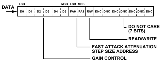
Figure 50. 16-Bit SPI Register
