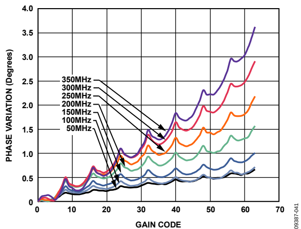
Figure 44. Phase Variation vs. Gain Code
