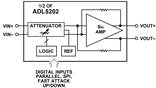
Figure 53. Simplified Schematic
