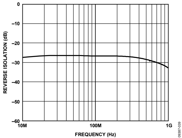
Figure 42. Reverse Isolation vs. Frequency
