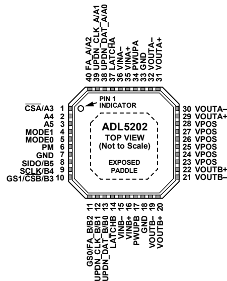
Figure 5. Pin Configuration
