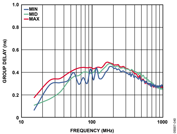
Figure 43. Group Delay vs. Frequency at Max, Mid, and Min Gain Outputs
