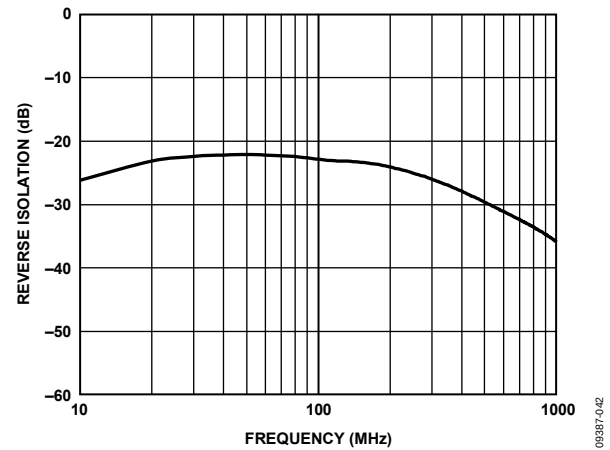
Figure 45. Disable-State Reverse Isolation vs. Frequency
