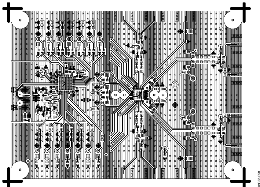
Figure 64. Evaluation Board Top Layer
