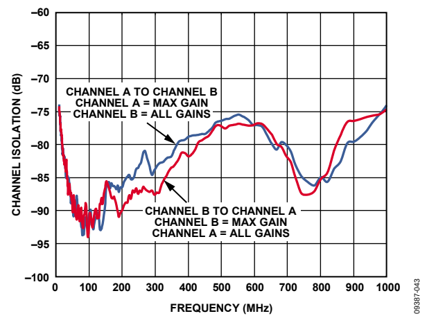
Figure 41. Channel Isolation vs. Frequency
