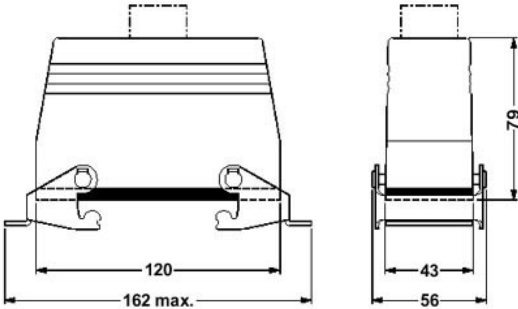
Dimensioned drawing
