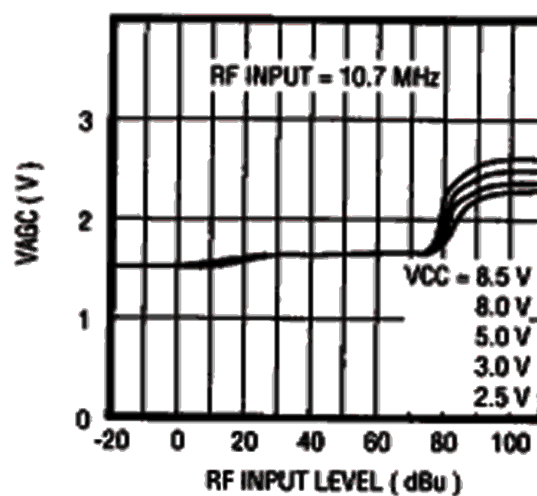
VAGC CHARACTERISTICS
