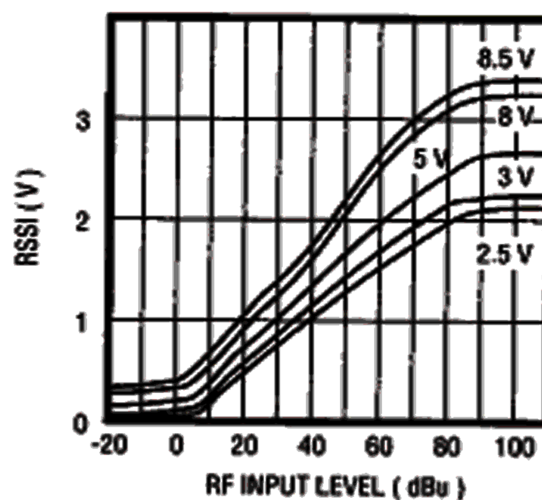
RSSI CHARACTERISTICS
