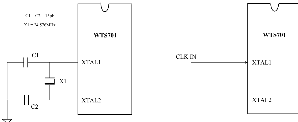
Figure 6. Clock Generation.
