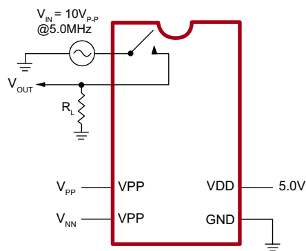
OFF Isolation
