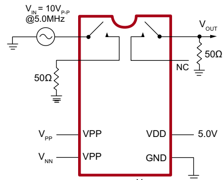
Crosstalk
