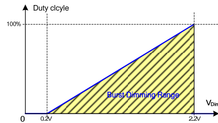
Figure3: Duty cycle of positive internal burst vs DIM voltage
