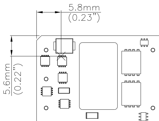
Figure 20: Temperature measurement location The allowed maximum hot spot temperature is defined at 118 °C.
