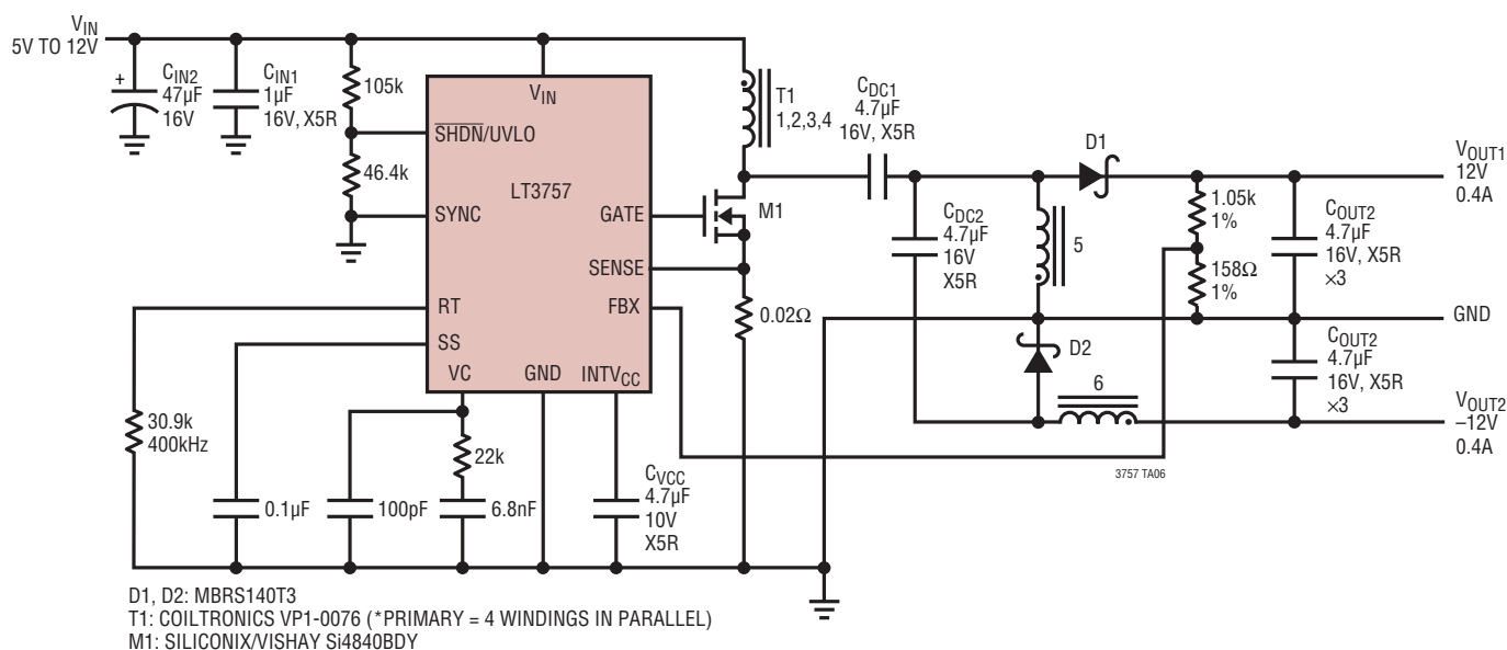
5V to 12V Input, \pm 12\text{V}/0.2\text{A} Output SEPIC Converter
