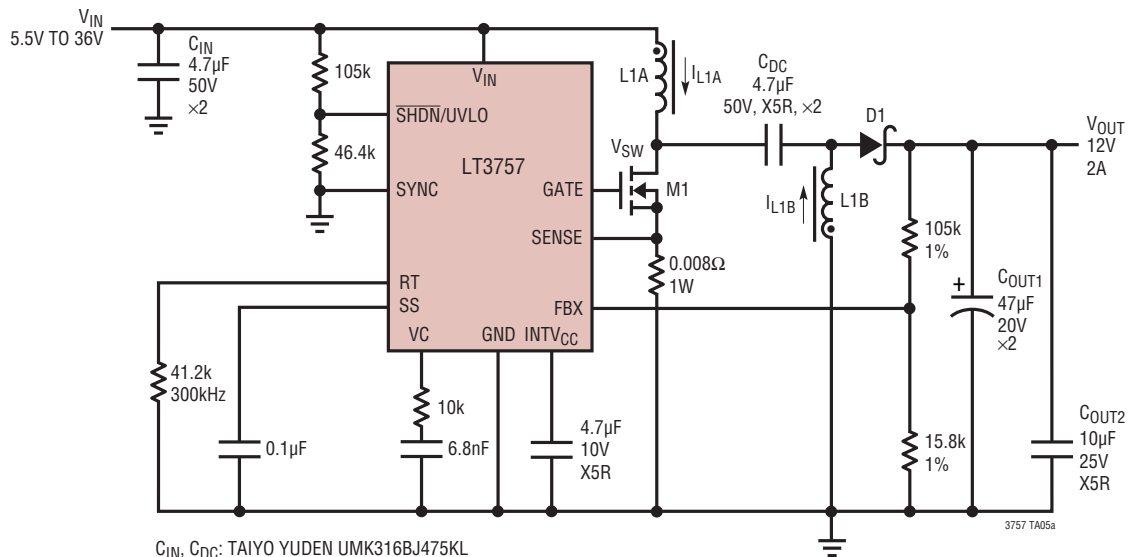
5.5V to 36V Input, 12V/2A Output SEPIC Converter
