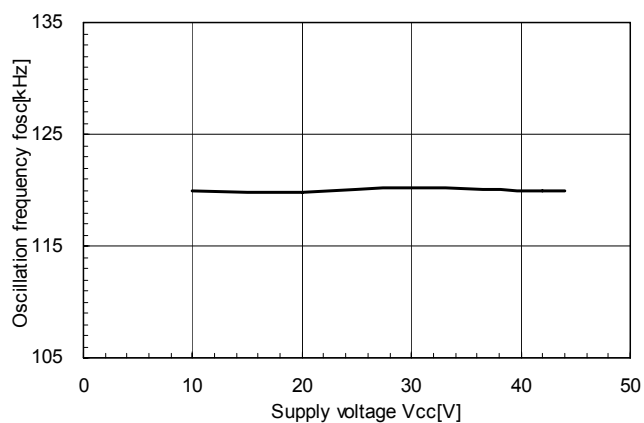
Oscillation frequency vs. Supply voltage VCC
