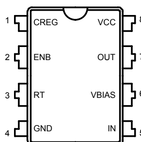
FA7764P(DIP-8)
