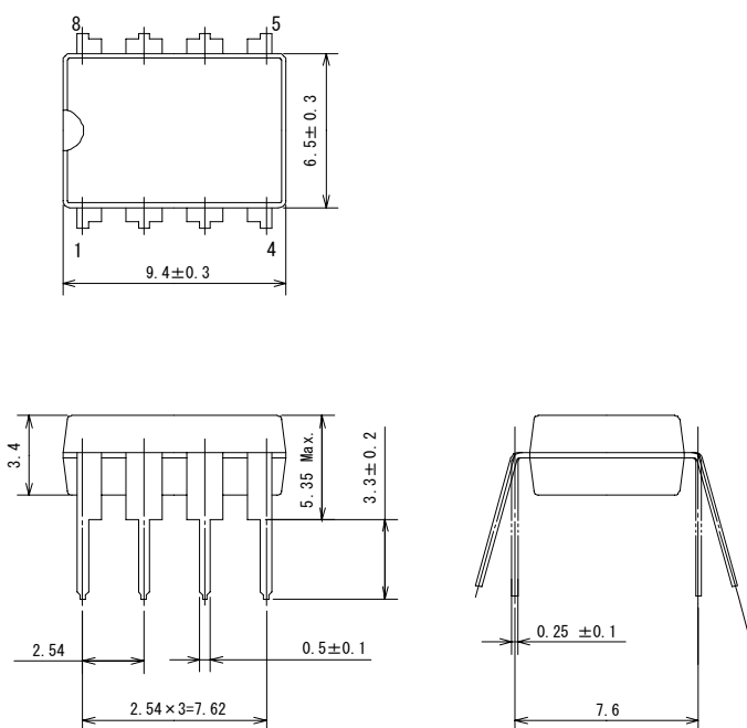
• FA7764P(DIP-8)
