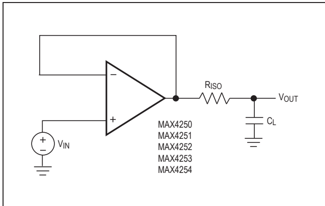
Figure 3. Overdriven Input Showing No Phase Reversal
