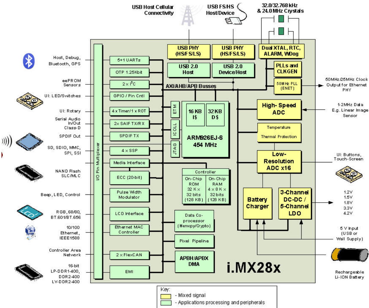
Figure 1. i.MX28 Simplified Interface Block Diagram
