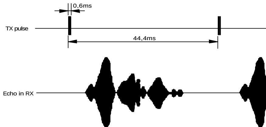
Fig. 1 - Pulse/Echo Timing
