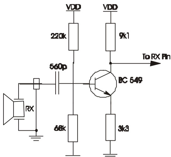
Fig. 4 - Recommended pre-amplifier
