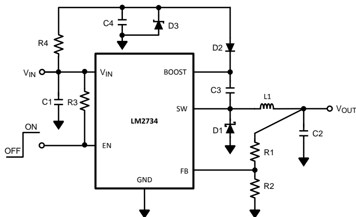
Figure 12. V BOOST Derived from V SHUNT 18V to 1.5V/1A
