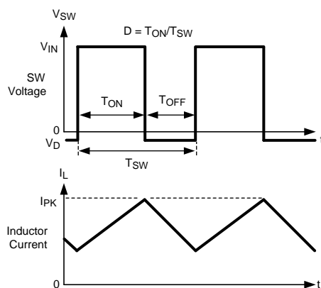
Figure 3. LM2734Z Waveforms of SW Pin Voltage and Inductor Current
