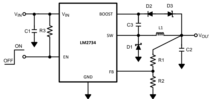
Figure 14. V_{BOOST} Derived from Series Zener Diode ( V_{OUT} ) 15V to 9V/1A
