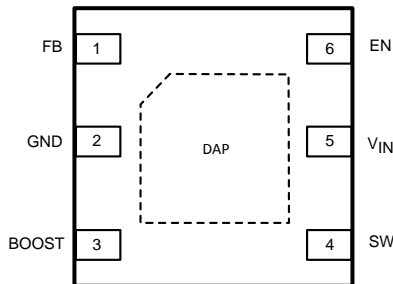
Figure 2. 6-Lead LLP (3mm x 3mm) NS Package Number SDE06A
