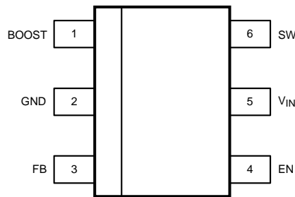
Figure 1. 6-Lead TSOT NS Package Number MK06A
