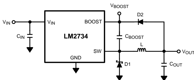
Figure 4. V_{OUT} Charges C_{BOOST}
