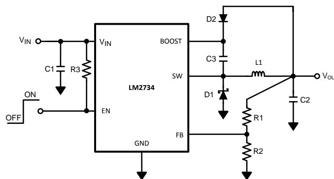
Figure 11. V_{\text{BOOST}} Derived from V_{\text{OUT}} 12V to 3.3V/1A
