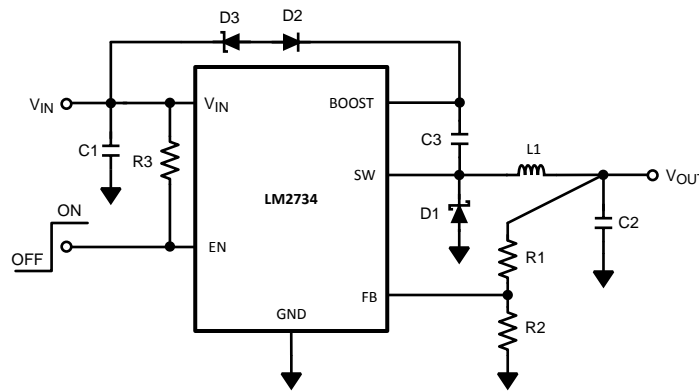
Figure 13. V_{BOOST} Derived from Series Zener Diode ( V_{IN} ) 15V to 1.5V/1A
