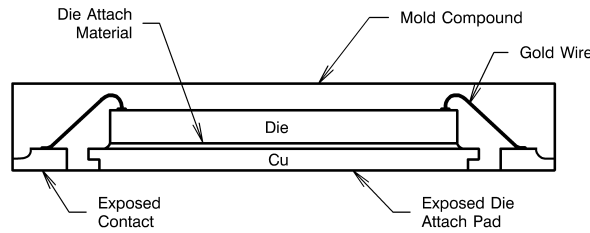
Figure 8. No Pullback LLP Configuration
