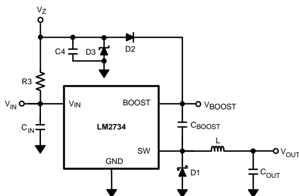
Figure 6. Boost Voltage Supplied from the Shunt Zener on V_{IN}
