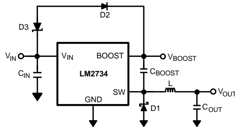
Figure 5. Zener Reduces Boost Voltage from V_{IN}
