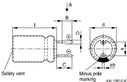
View A
