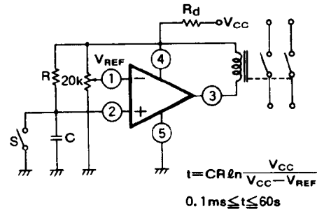
(2) CR Timer
