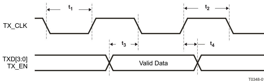
Figure 9-11. 10 Mb/s MII Transmit Timing
