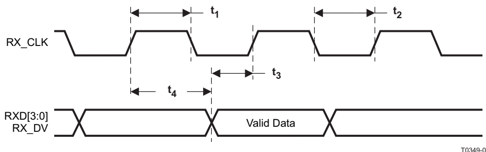
Figure 9-12. 10Mb/s MII Receive Timing
