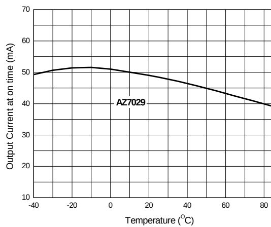
Figure 9. Output Current at on Time vs. Temperature
