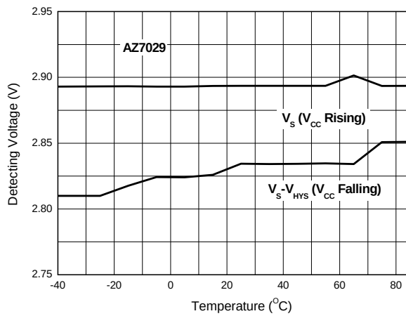
Figure 7. Detecting Voltage vs. Temperature
