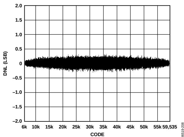
Figure 20. DNL Plot
