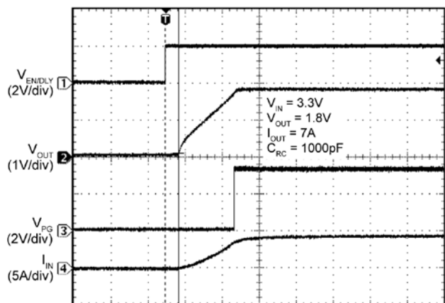
Enable Turn-On Delay/Rise Time
