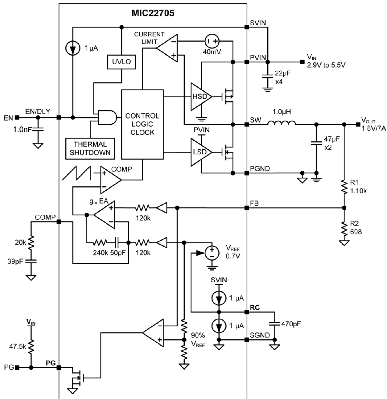
Figure 1. MIC22705 Functional Diagram
