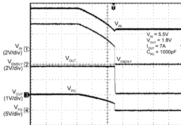
V IN Turn-Off
