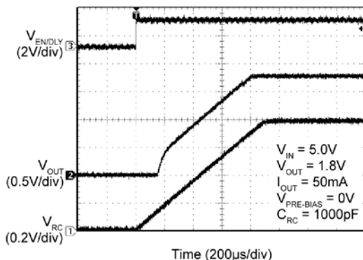
Figure 3. EN Turn-On Time – Normal Start-Up
