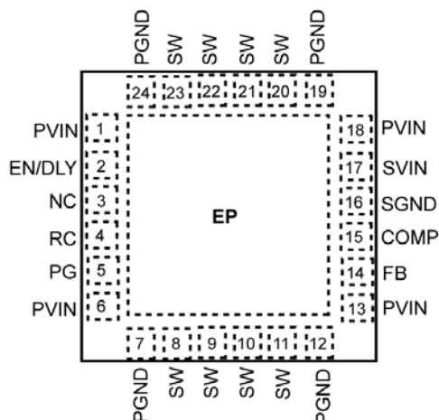
24-Pin 4mm × 4mm MLF ® (ML)
