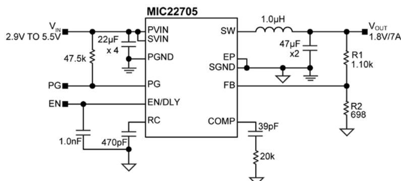
MIC22705 7A 1MHz Synchronous Output Converter
