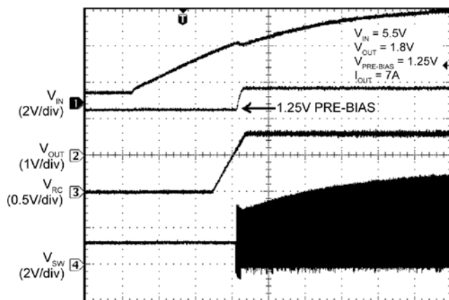
V IN Start-Up with Pre-Biased Output
