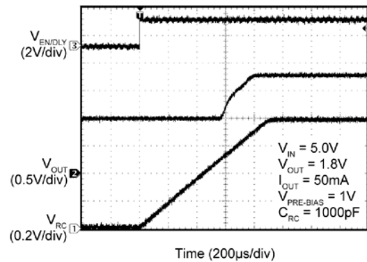
Figure 4. EN Turn-On at 1V Pre-Bias
