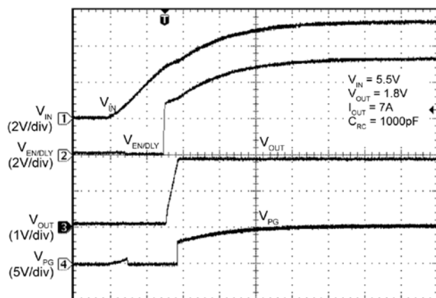
V IN Turn-On
