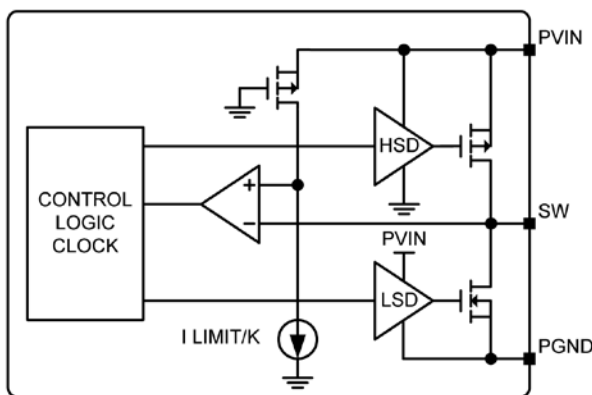
Figure 7. Current-Limit Detail
