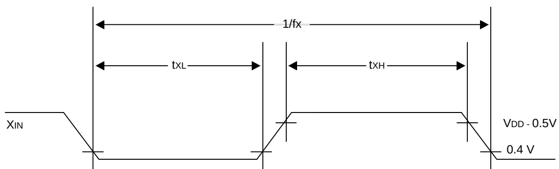
Figure 14-5. Clock Timing Measurement at X_{IN}
