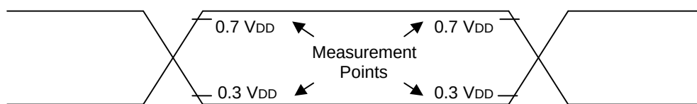
Figure 14-4. A.C. Timing Measure Points (Except for X_{IN} )
