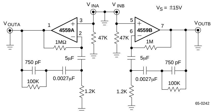
Figure 21. RIAA Preamplifier
