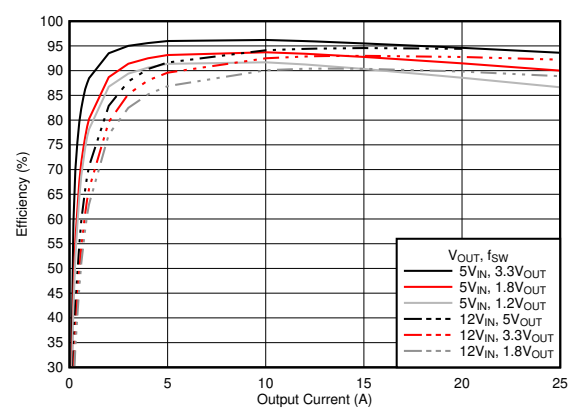
Typical Efficiency
