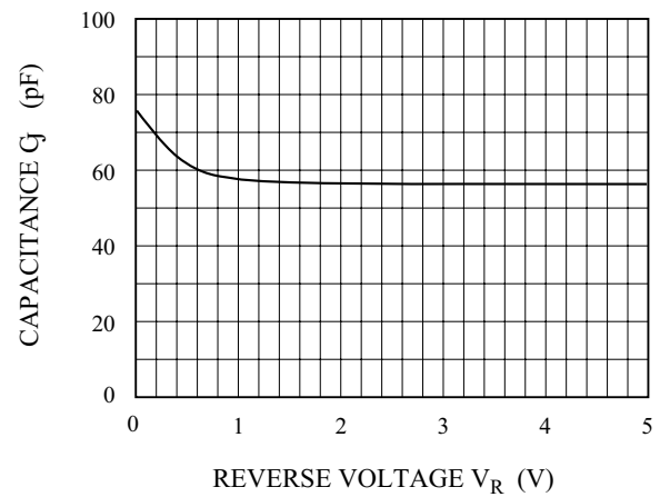
C_J - V_R
